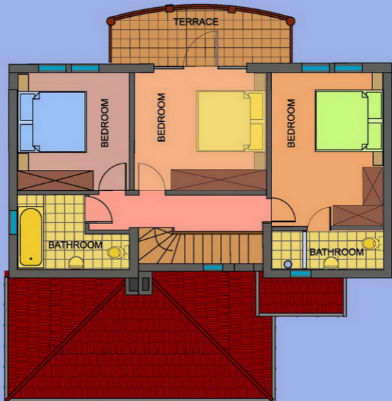
Second floor with 3 bedrooms - option 1
